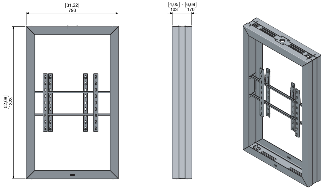
Technical drawing (mm/inch) Casing Complete Top Mounted Back to Back 55"
