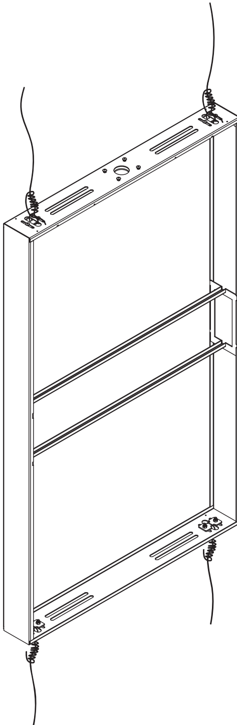
Support cable
