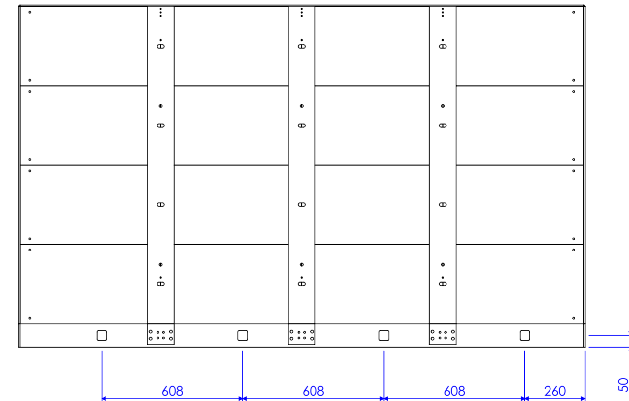
REAR VIEW CABLE HOLES
