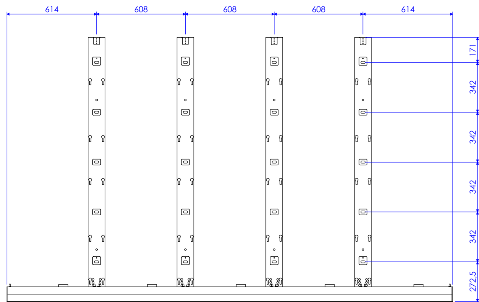
FRONT VIEW MOUNTING
