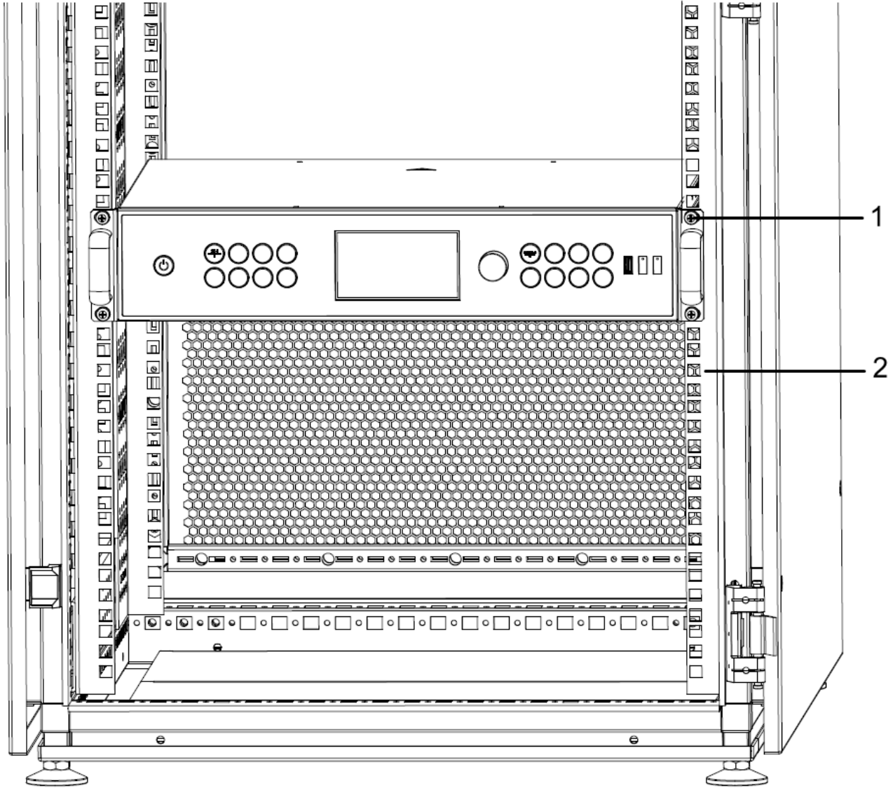
Figure 2-8 Install the DT90 Device in the Rack
