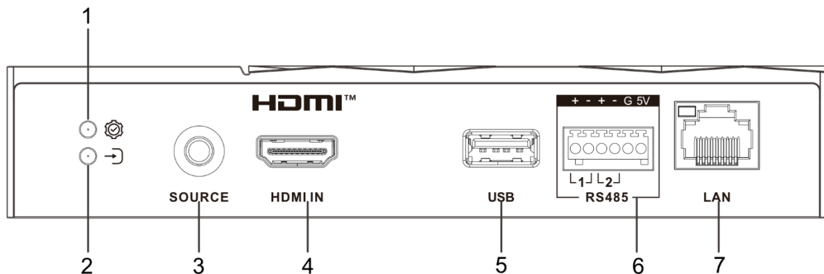
Figure 1-1 DT30 Series Device Front Panel
