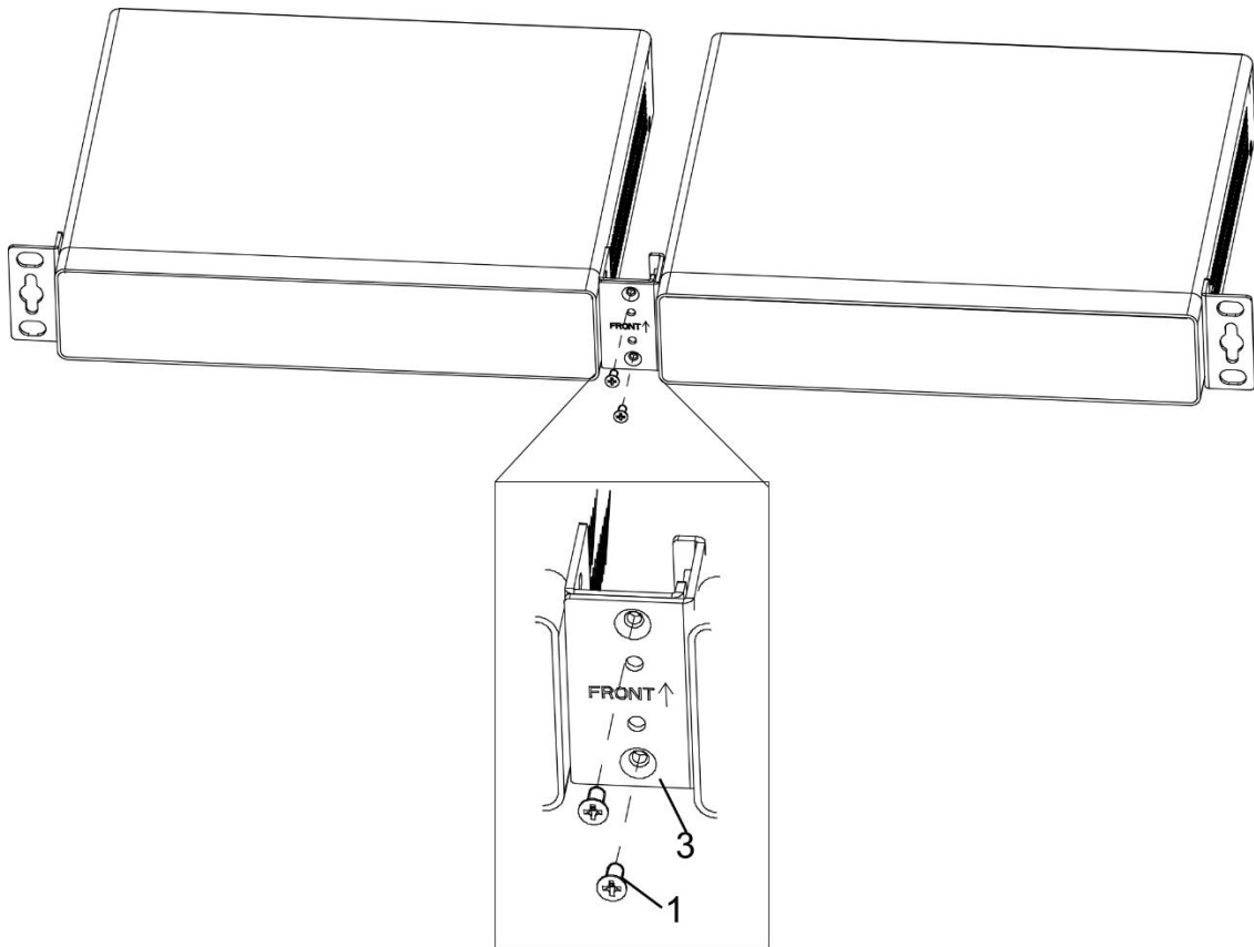
Figure 2-5 Secure the Connecting Brackets
