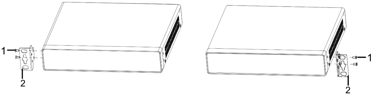
Figure 2-3 Install the Mounting Ears
