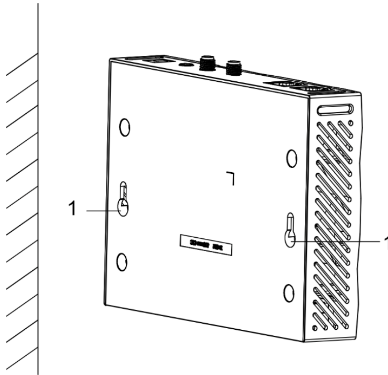
Figure 2-2 Wall Mounting
