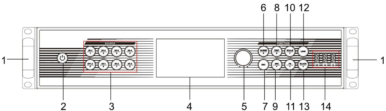
Figure 1-7 DT90 Series Device Front Panel
