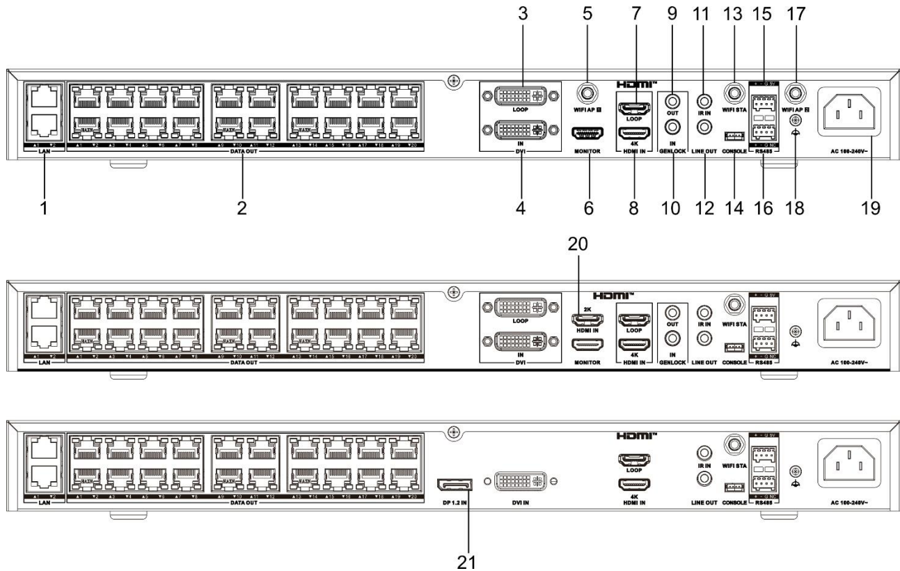
Figure 1-6 DT60 Series 4K Device Rear Panel
