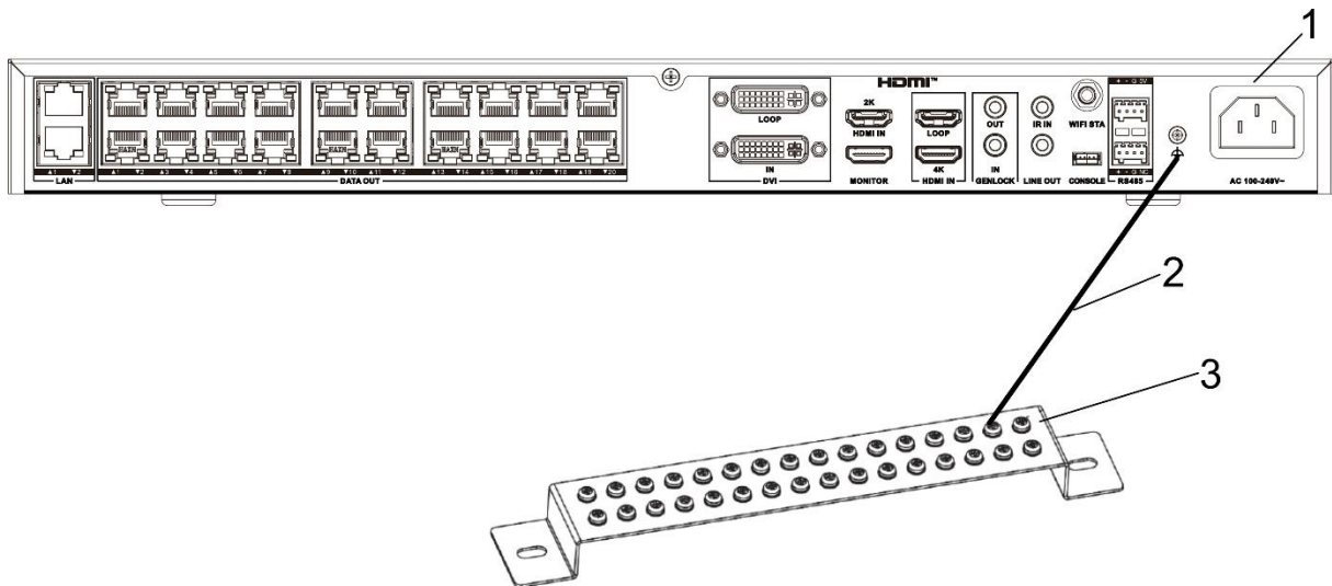
Figure 2-9 Connect the Ground wire to the Grounding Busbar
