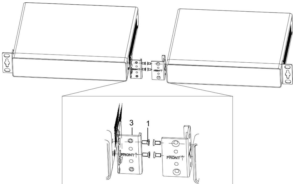
Figure 2-4 Install the Connecting Brackets
