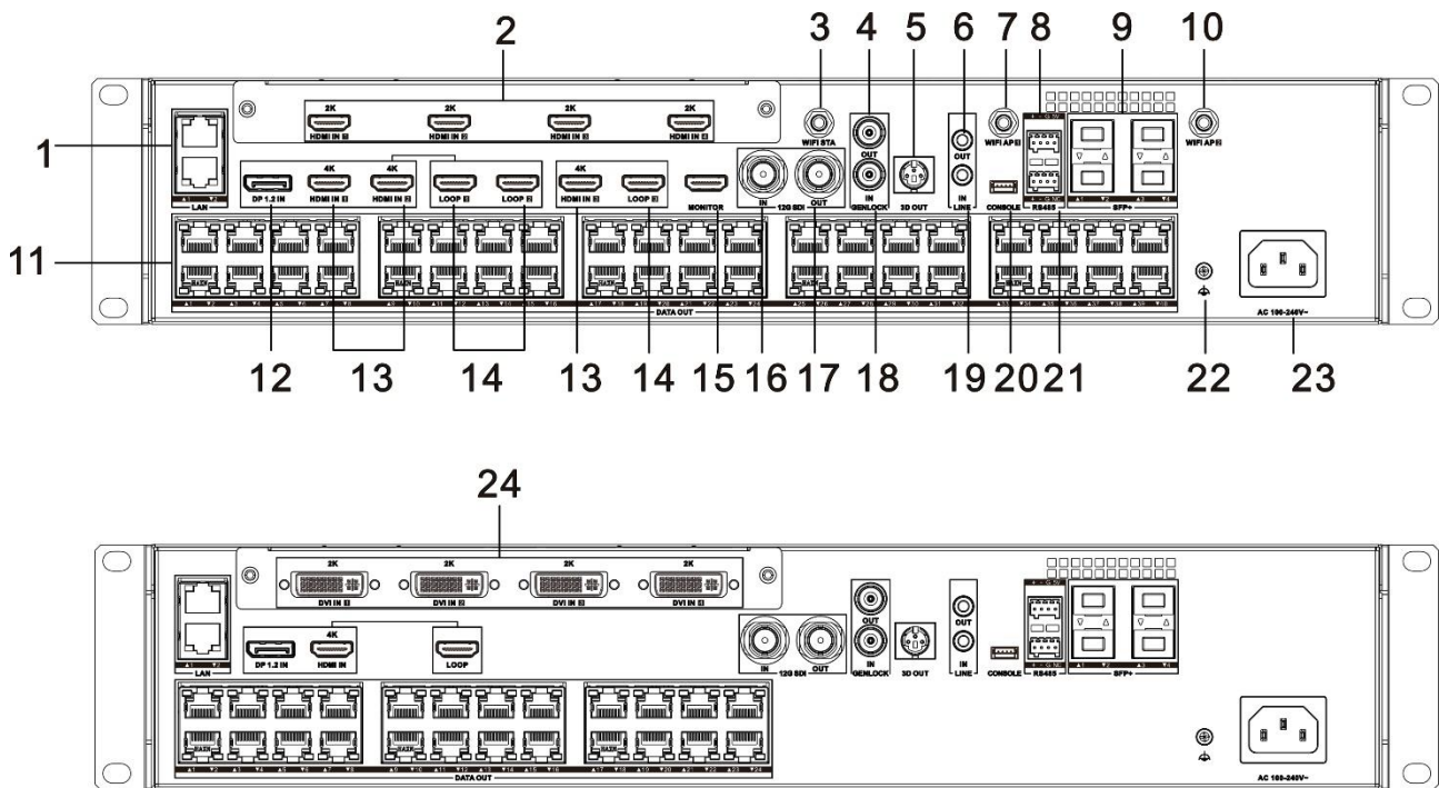
Figure 1-8 DT90 Series Device Rear Panel
