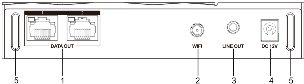
Figure 1-2 DT30 Series Device Rear Panel
