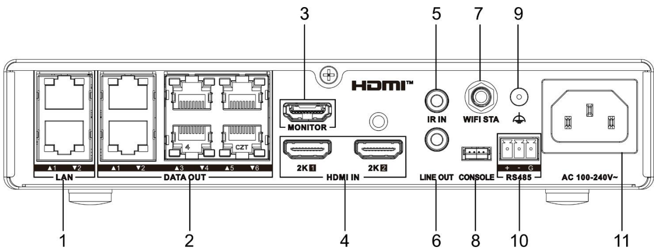
Figure 1-4 DT60 Series 2K Device Rear Panel
