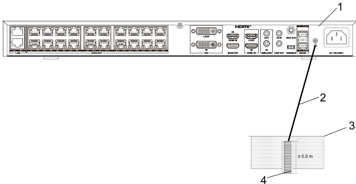
Figure 2-10 Connect the Ground wire to the Grounding Electrode
