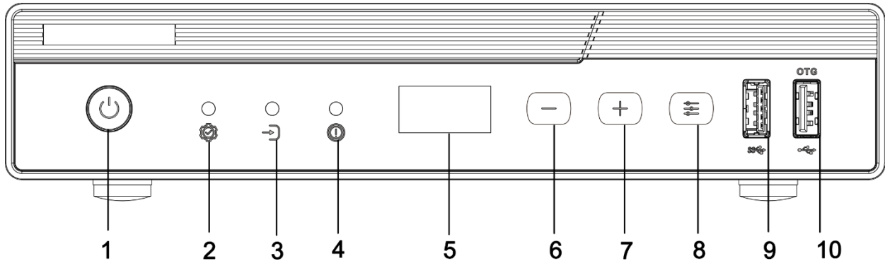
Figure 1-3 DT60 Series 2K Device Front Panel
