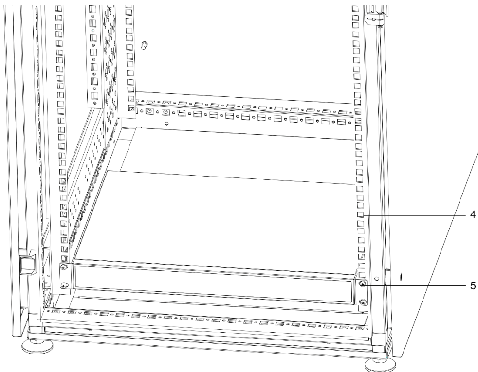
Figure 2-7 Install 4K Device in the Rack
