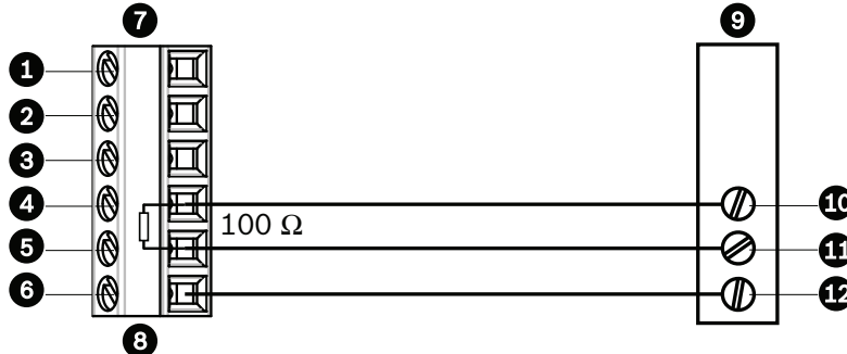
Figure 9.5: Connections for RS485 Operations
