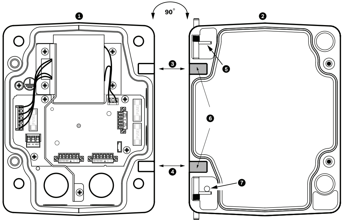
Figure 6.1: Align Cover Door Hinge to Power Box
