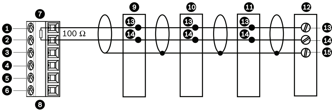
Figure 9.2: Connections for a Daisy Chain Configuration
