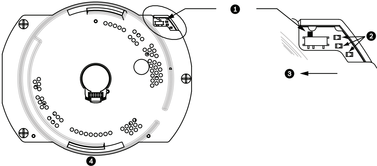
Figure 9.4: Position of CPU Switch for RS232 Operation (camera module not shown for clarity)
