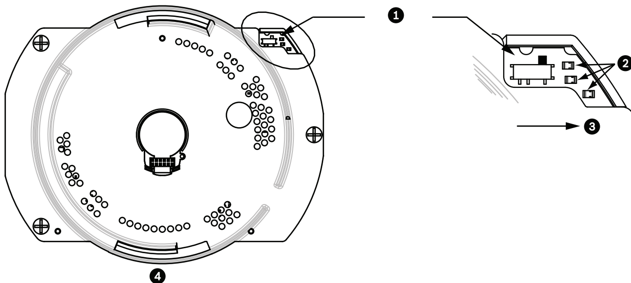
Figure 9.6: Position of CPU Switch for RS-485 Operation (camera module not shown for clarity)
