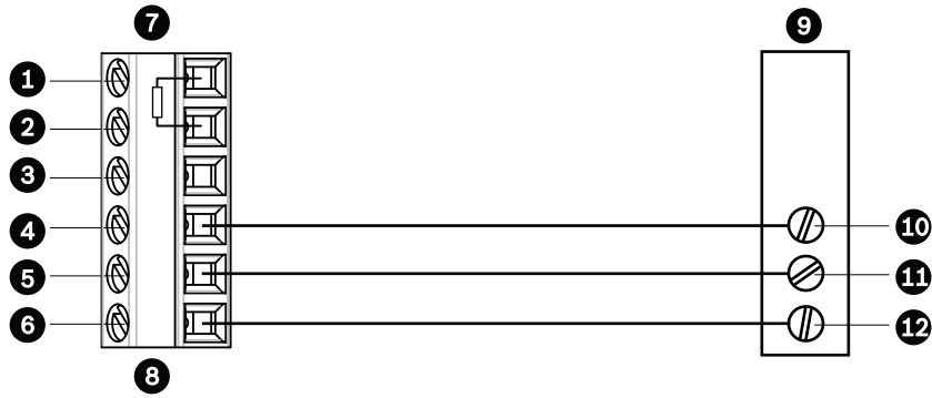
Figure 9.3: Connections for RS232 Operation
