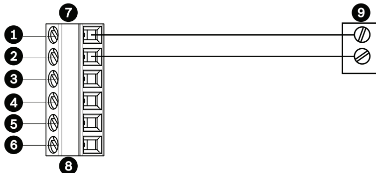
Figure 11.1: Connections for audio over an Ethernet network
