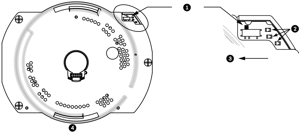
Figure 10.2: Position of CPU Switch for RS-232 Operation
