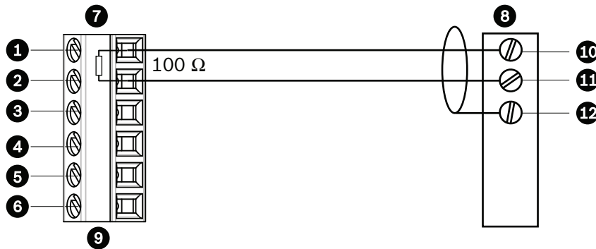
Figure 9.1: Connections for Biphase Operation
